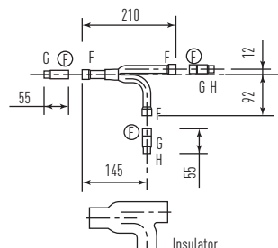
Dimensions for connections of each part
