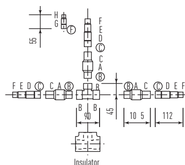
Dimensions for connections of each part
