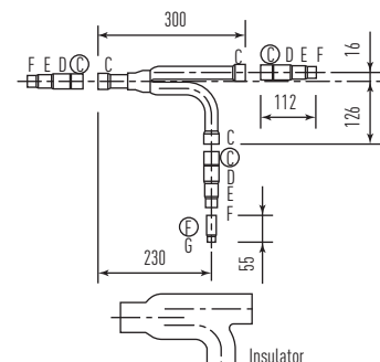
Dimensions for connections of each part
